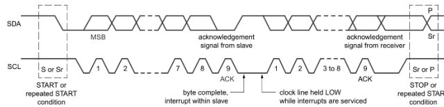
Figure 3 Data transfer on the I2C bus
